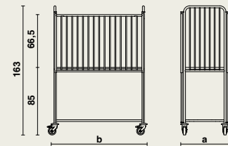
Dimensions for a fixed mattress platform
